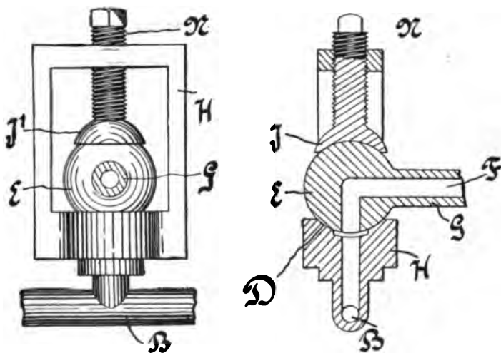
FIG. 319.—The Perrott Improved "Torch" Head. The frame, H, is permanently attached to the nipple of the regulator gasoline outlet at B. At its top, H carries the screw, N, with the cup-shaped clamp end, J. The spherical head, E, having the internal channel, F, is attached at the end of one leg of the "torch" by the neck, G. When the "torch" is heated and inserted in the burner space, the head, E, is placed in position, as shown, and secured by the screw clamp, so that the channel, F, connects direct with B, thus permitting gasoline to flow into the "torch" tubes. The particular advantages claimed are the absence of movable screw joints, which are apt to suffer from heat, and also the avoidance of all packing.
